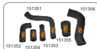
RK 151350 Price Rs. 1120.00 Hose Pipe Set (Set of 6 Pcs.) (1351+1352+1353+1354+1355+1356) Zetor 2522/3522
